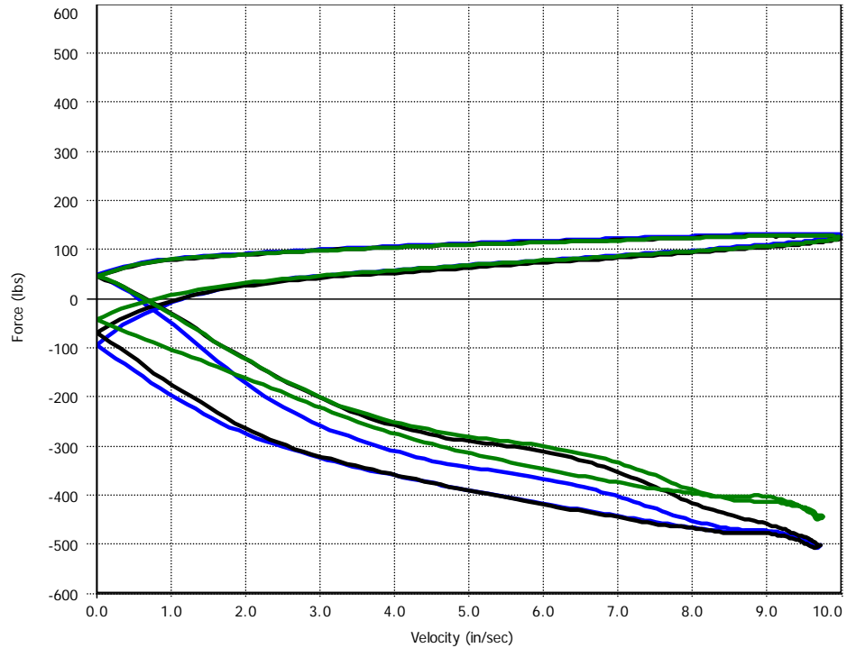
Figure 7. Comparison plot of LF damper from three different test days.
