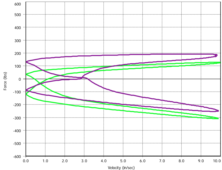
Figure 6. Comparison FV plot of RR shock tested at Haas and RR shock tested in house.
