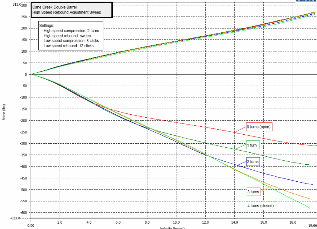
Figure 2. High Speed Rebound Adjustment Sweep
