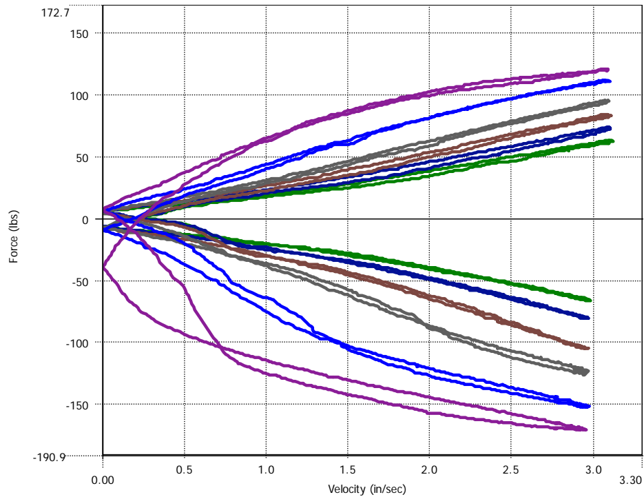
Figure 9. Double Barrel low-speed adjustability.
