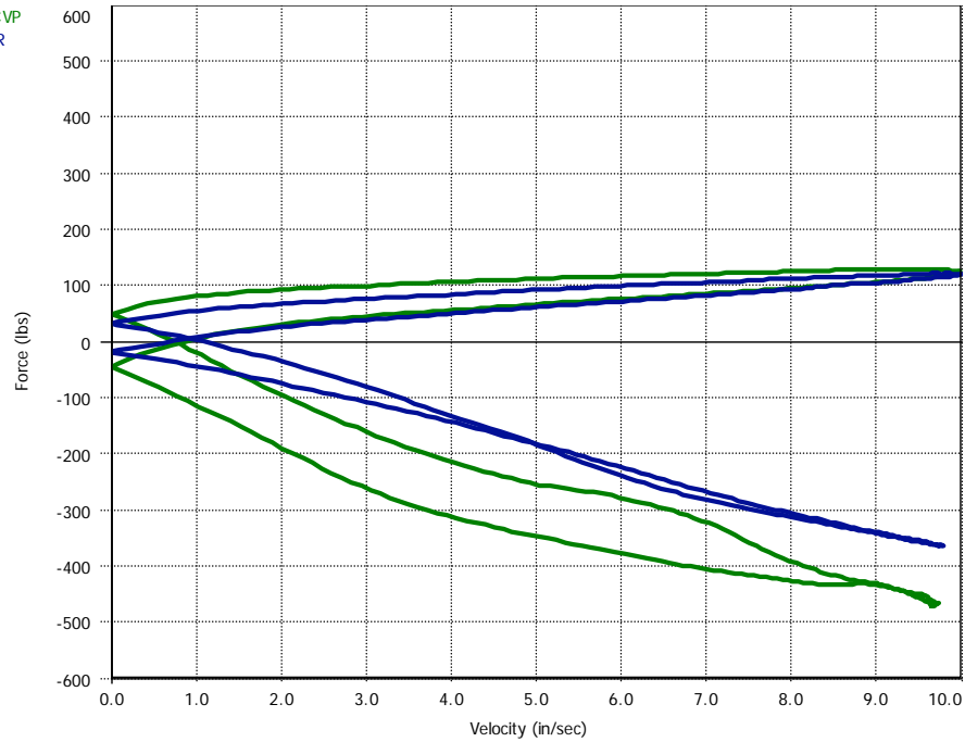
Figure 8. Comparison of LF damper before and after oil change and adjustment.
