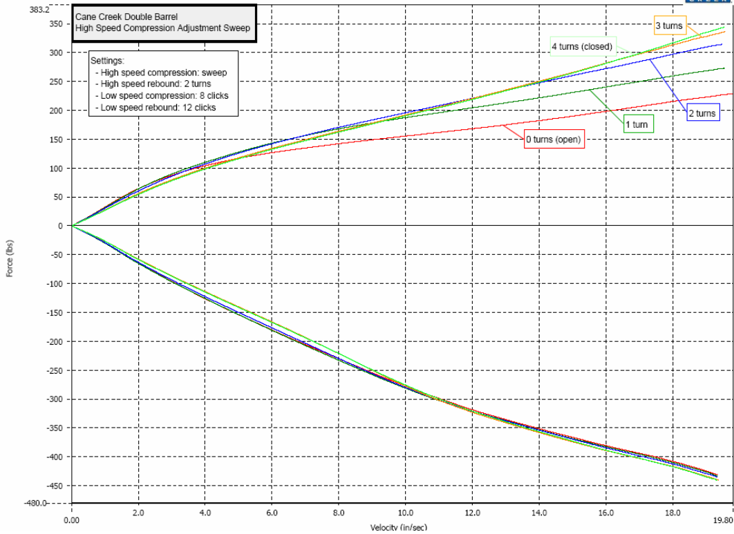
Figure 1. High Speed Compression Adjustment Sweep
